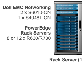
Figure 2: Dell EMC NFV Ready Bundle for VMware Rack Configuration
