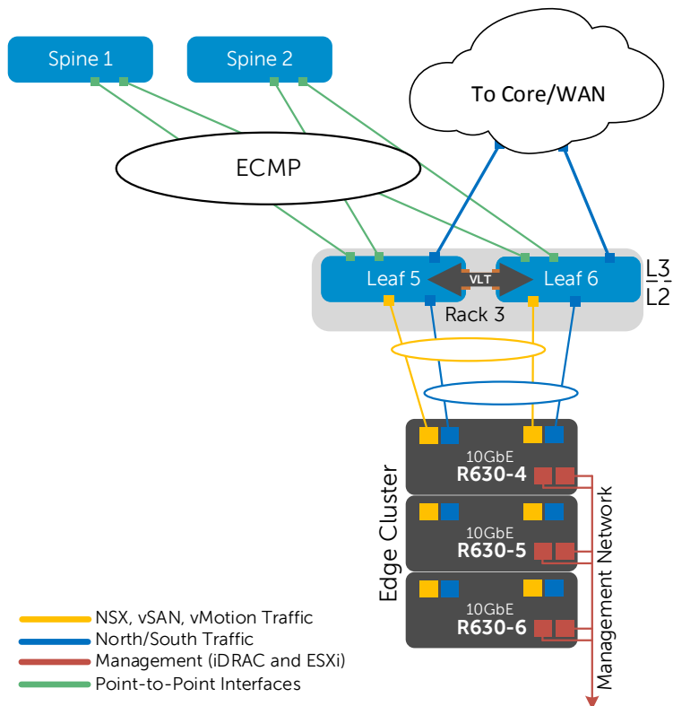
Figure 22 Edge cluster leaf switch configuration
