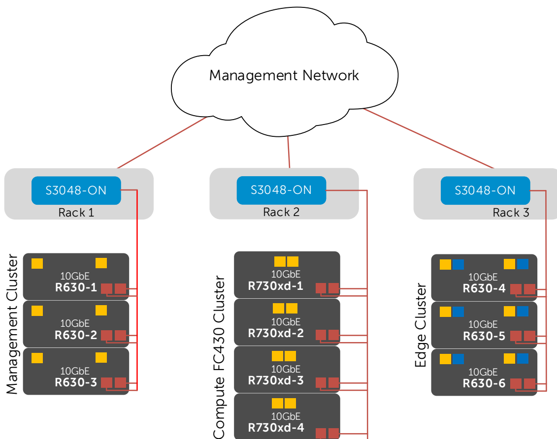
Figure 10 Physical layout of iDRAC and ESXi management interfaces
