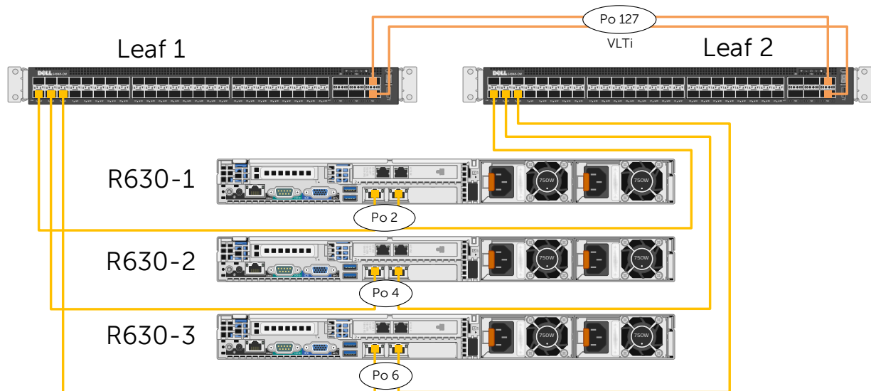
Figure 11 Production network connections for the management cluster
