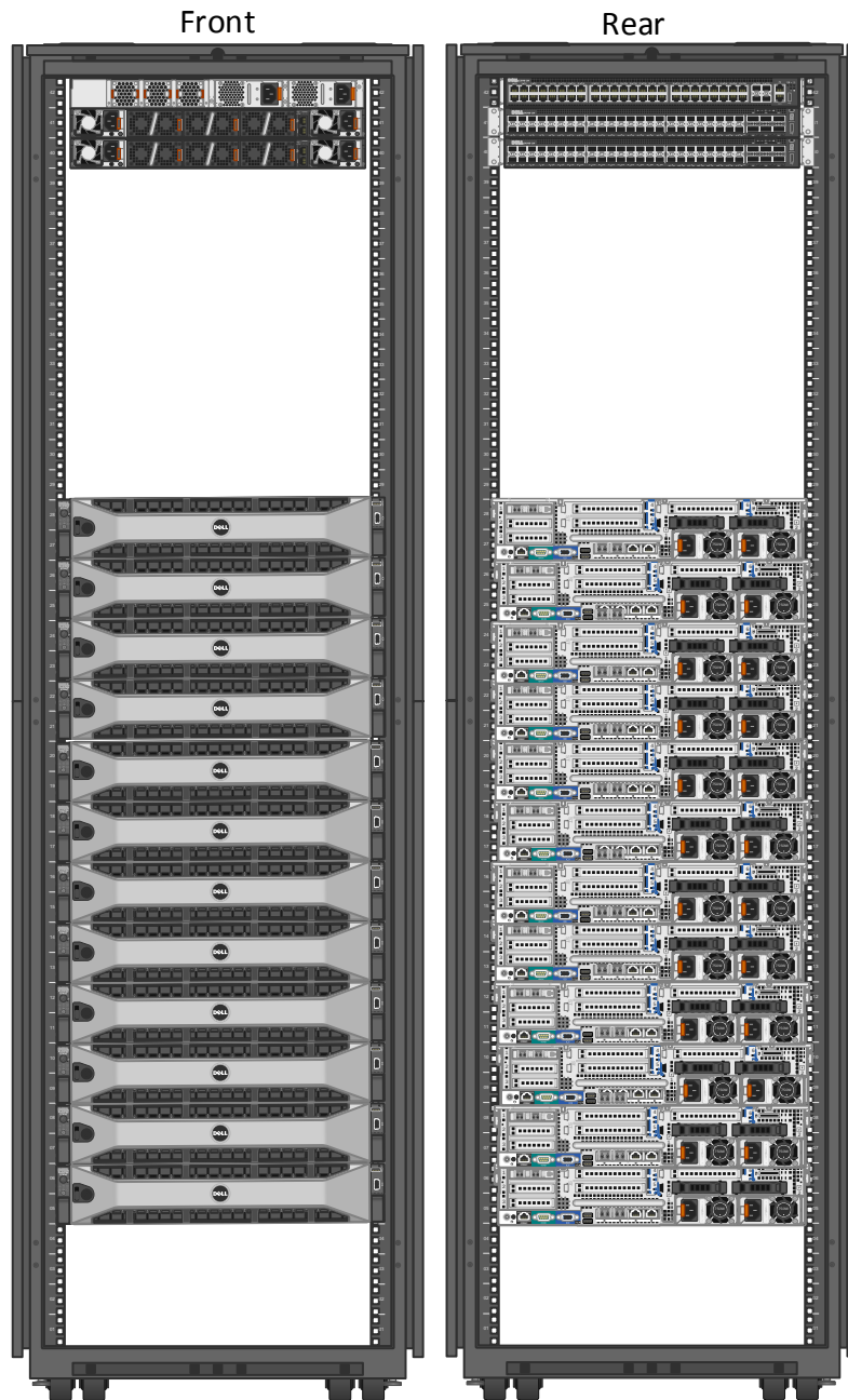
Figure 85 Rack containing compute cluster and switches
