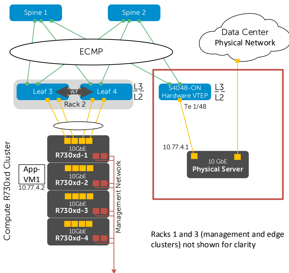
Figure 76 Hardware VTEP and physical server location in leaf-spine network
