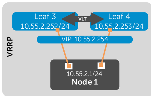
Figure 20 VRRP configuration example – VLAN 55 in Rack 2
