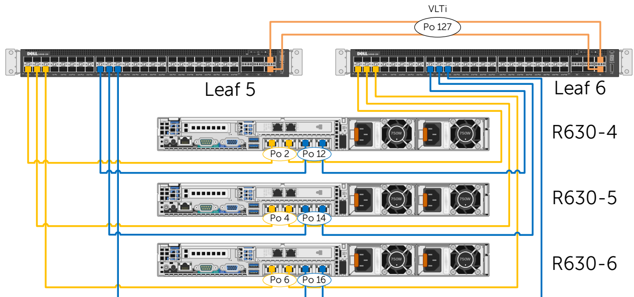
Figure 13 Production network connections for the edge cluster
