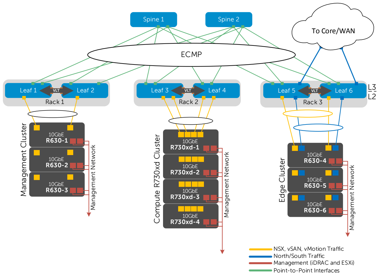
Figure 7 Physical production network
