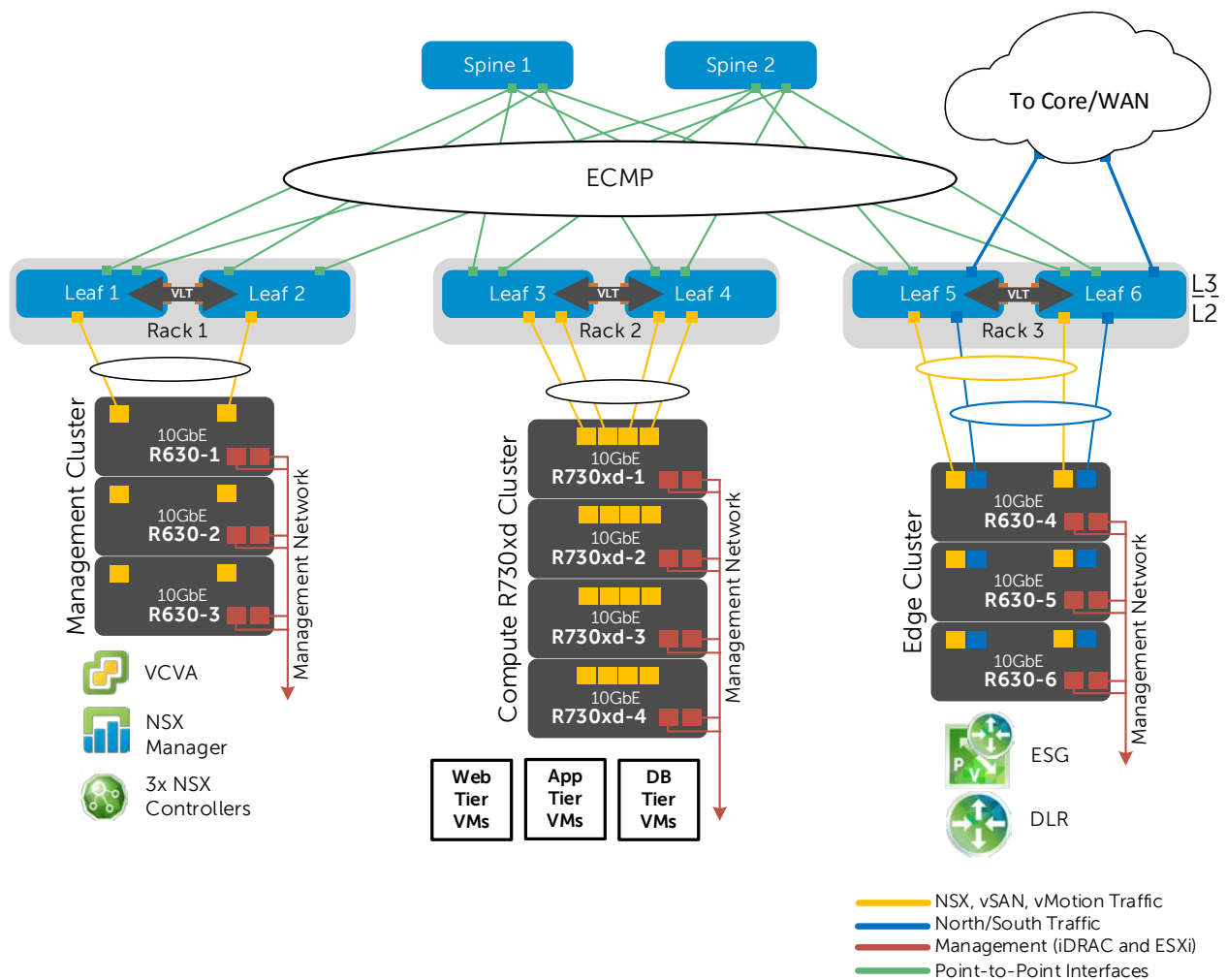
Figure 9 Combined physical and virtual networks
