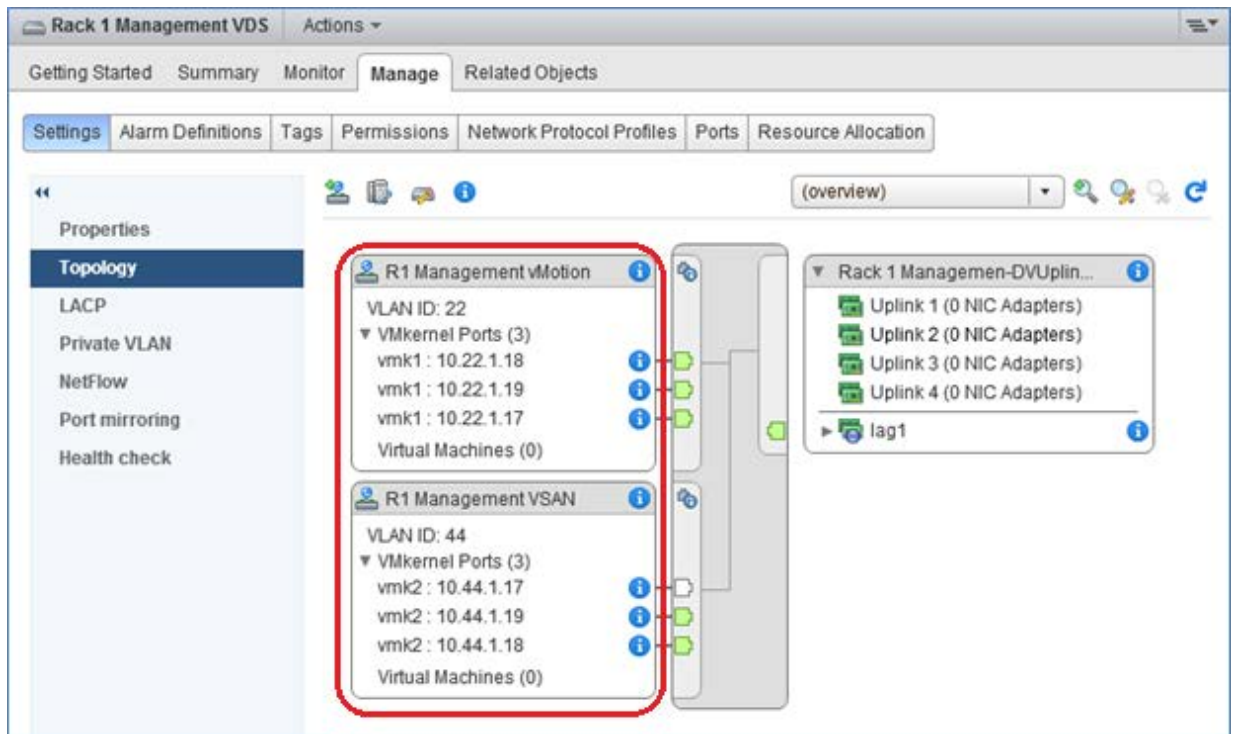
Figure 39 Rack 1 Management VDS VMkernel ports, VLANs, and IP addresses
