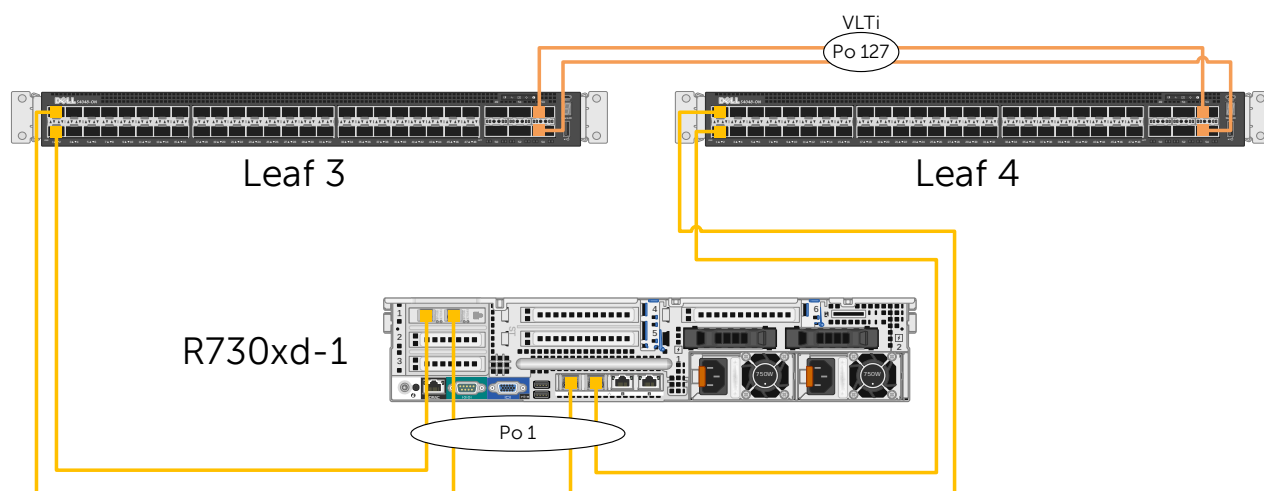
Figure 12 Production network connections for R730xd-1 in the compute cluster
