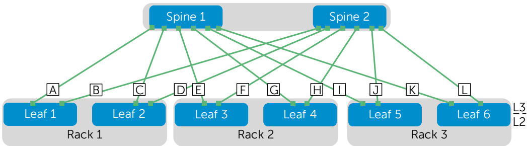
Figure 19 Point-to-point IP addressing
