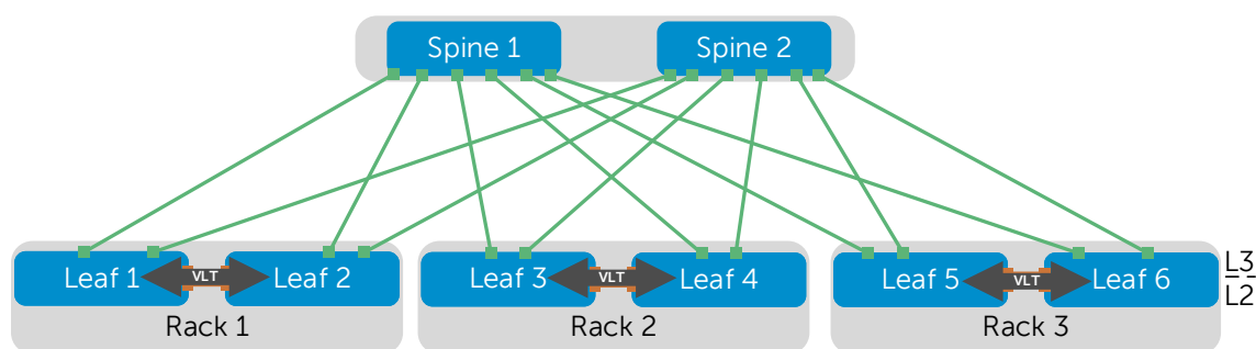
Figure 16 Spine and leaf topology example
