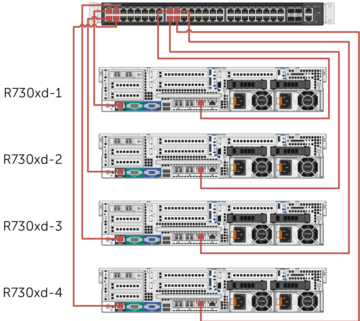
Figure 15 Compute cluster – management network connections
