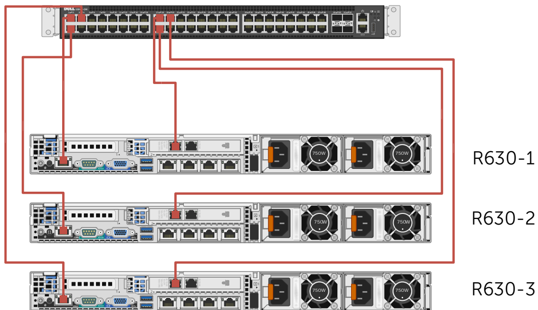
Figure 14 Management cluster – management network connections (edge cluster is identical)
