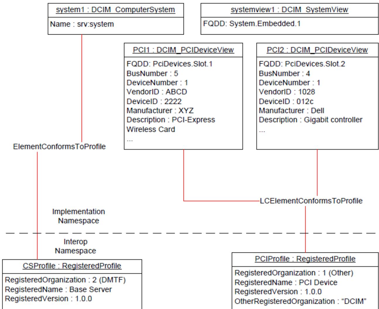
Figure 2. PCI Device Profile Implementation
