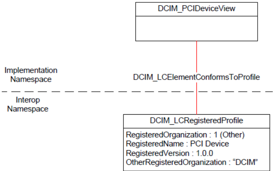
Figure 1. Class Diagram
