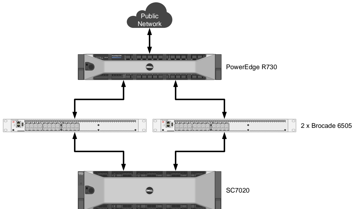
Figure 1 Single server reference architecture
