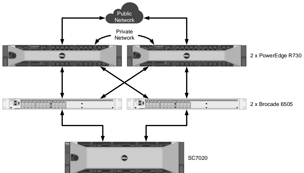
Figure 2 Highly available reference architecture
