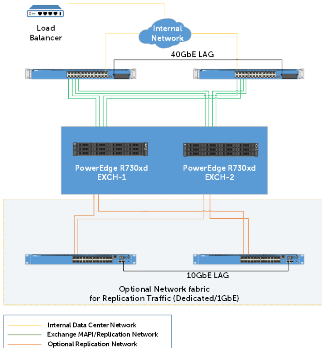
Figure 8 Complete network architecture for the Exchange reference implementation
