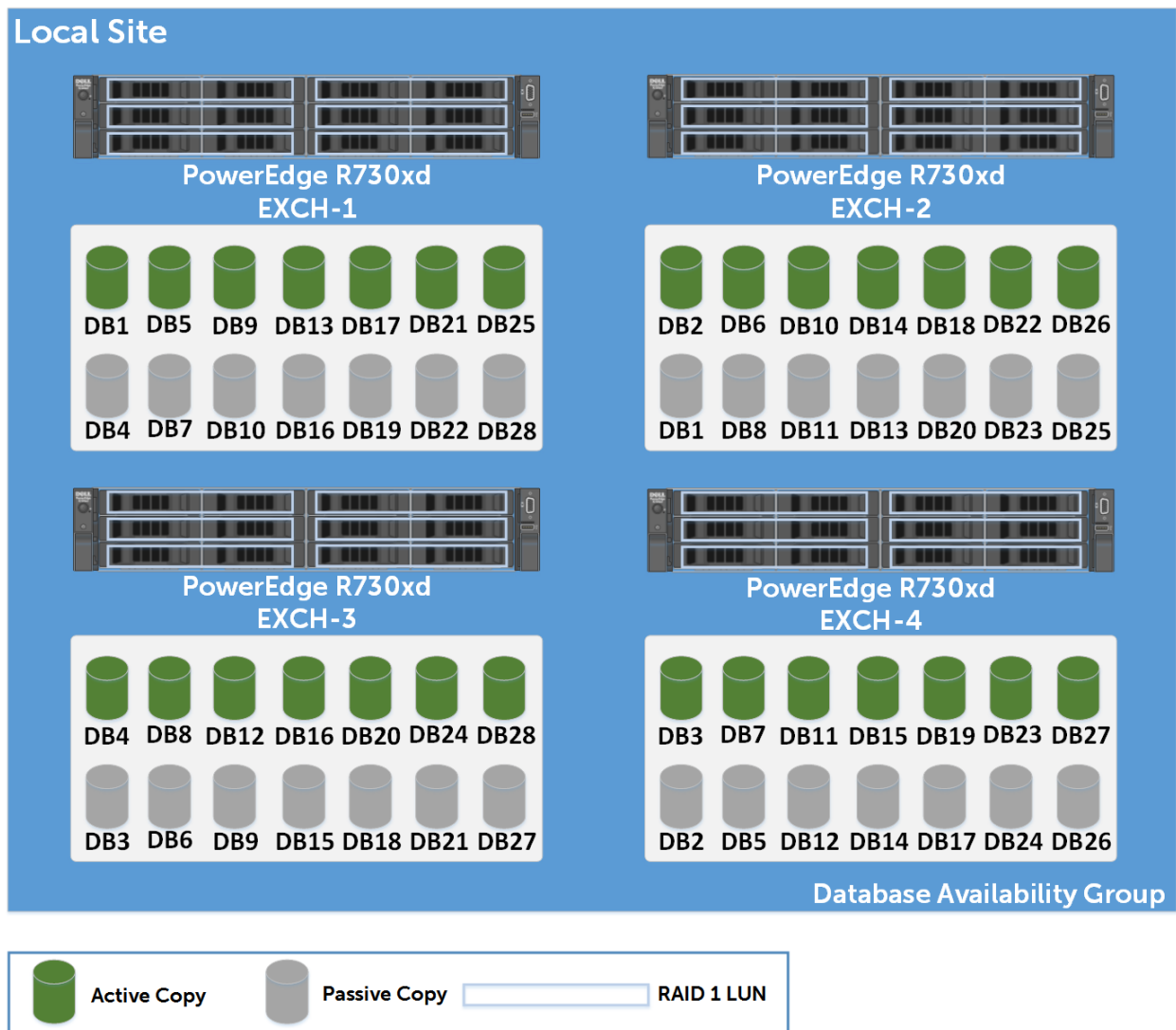
Figure 7 Exchange database layout in the reference implementation
