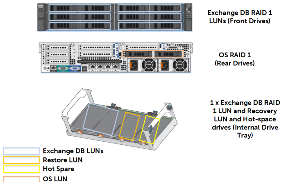
Figure 4 RAID LUN layout for the Exchange databases
