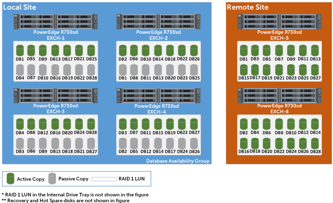
Figure 10 Exchange DAG architecture for the reference implementation
