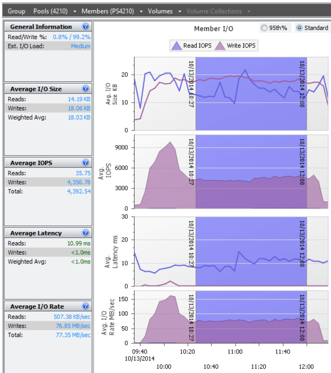
Figure 7 SAN HQ data showing steady state I/O for PS4210XS array
