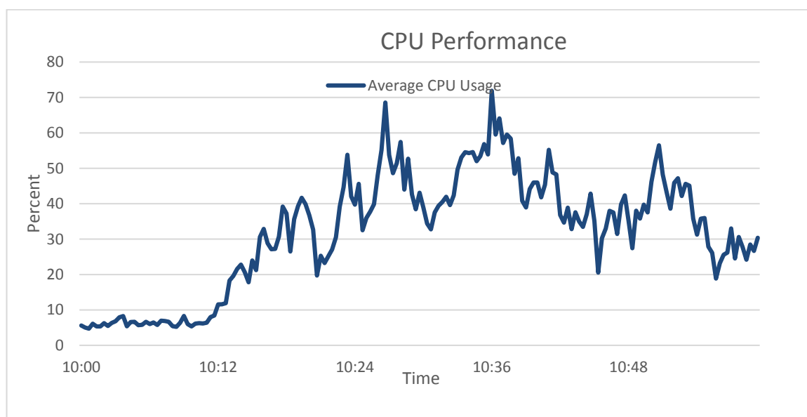
Figure 8 Average CPU performance per core on one vSphere host during login storm and steady state
