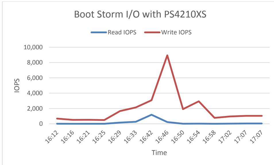
Figure 5 SAN HQ data showing boot storm performance with PS4210XS array
