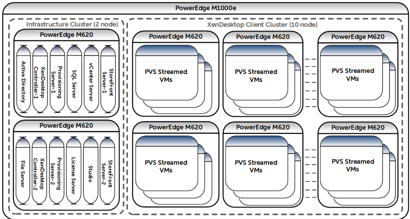
Figure 3 vSphere blade clusters
