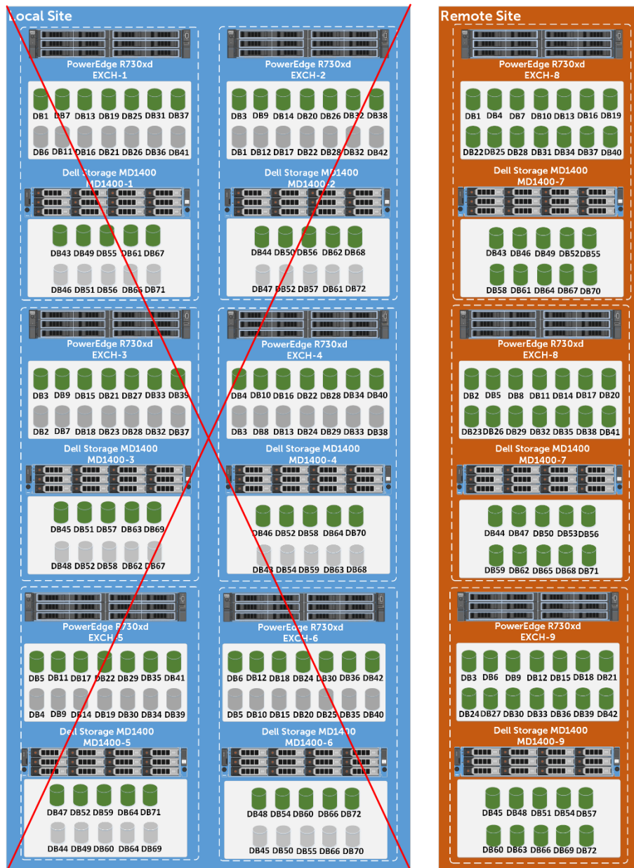
Figure 10 Exchange DAG architecture for the reference implementation
