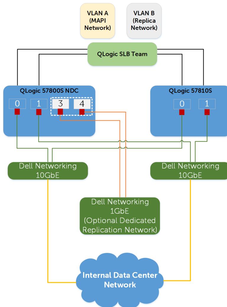
Figure 6 Network architecture for the Exchange deployment
