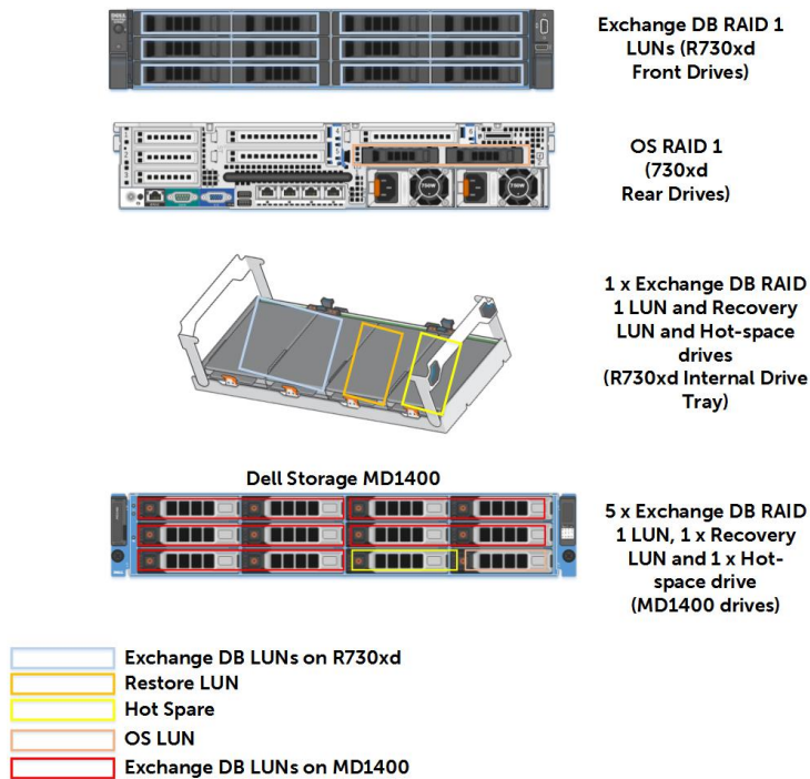
Figure 4 RAID LUN layout for the Exchange databases
