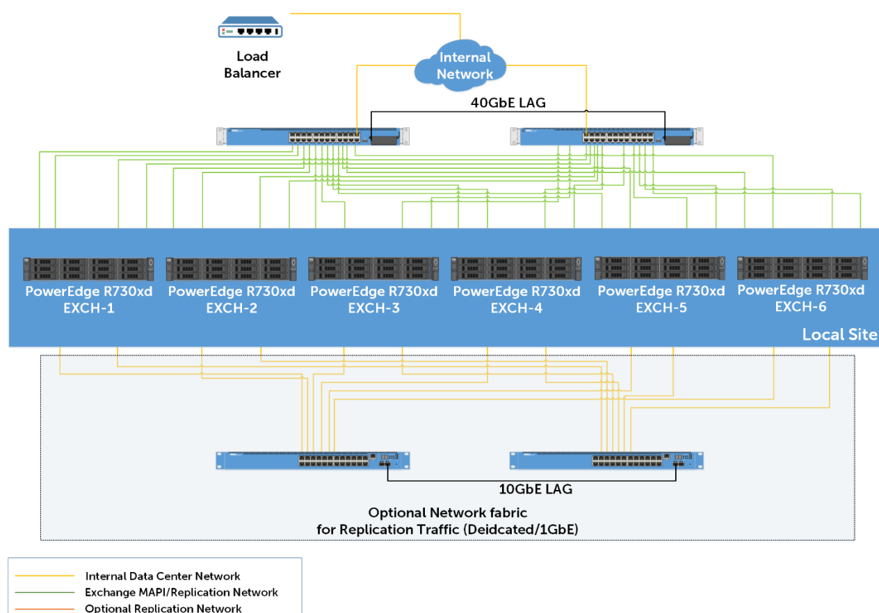
Figure 8 Complete Network Architecture for the Exchange reference implementation
