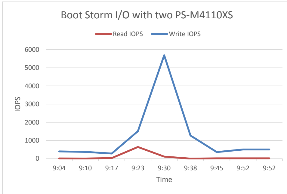
Figure 5 SAN HQ data showing boot storm performance with two PS-M4110XS arrays
