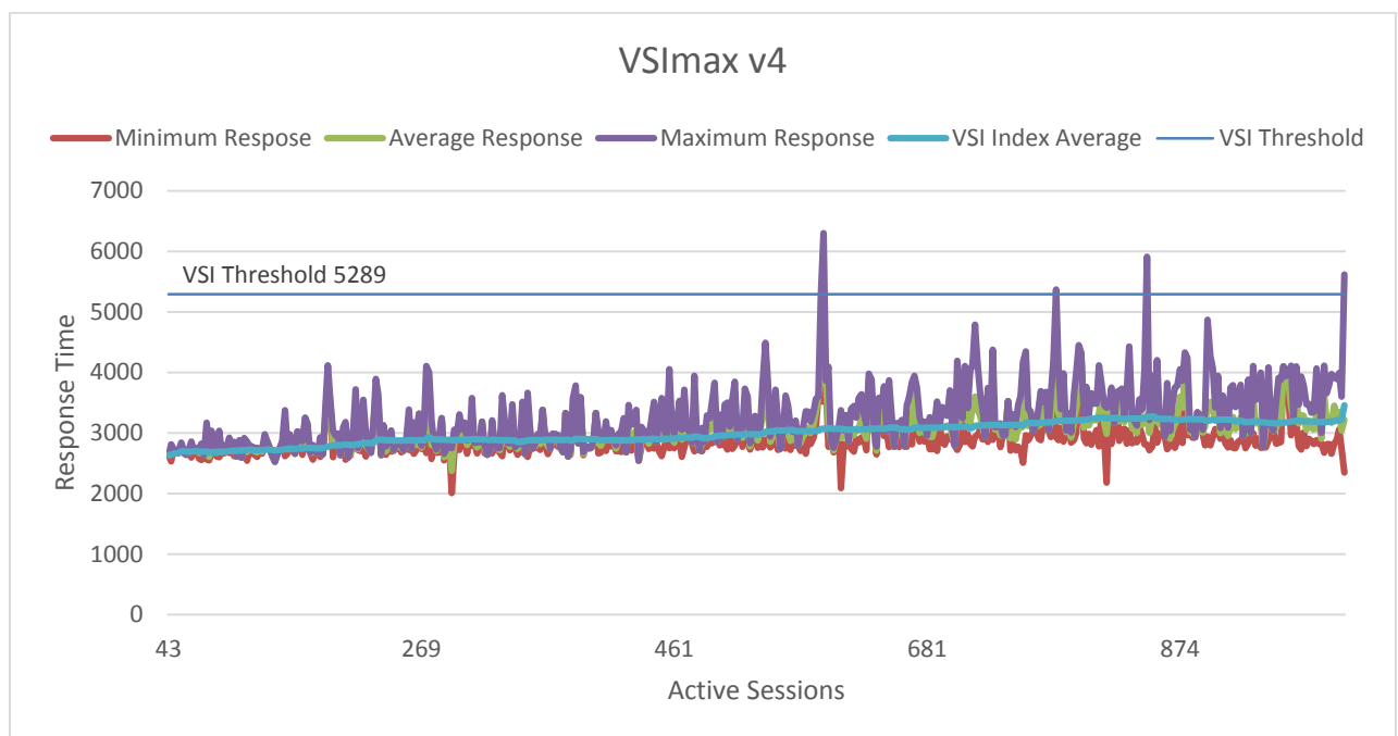
Figure 16 Login VSI generated graph showing average response time per user and VSImax for 1,000 VMs
