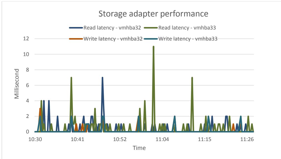
Figure 11 Storage adapter performance during login storm and steady state
