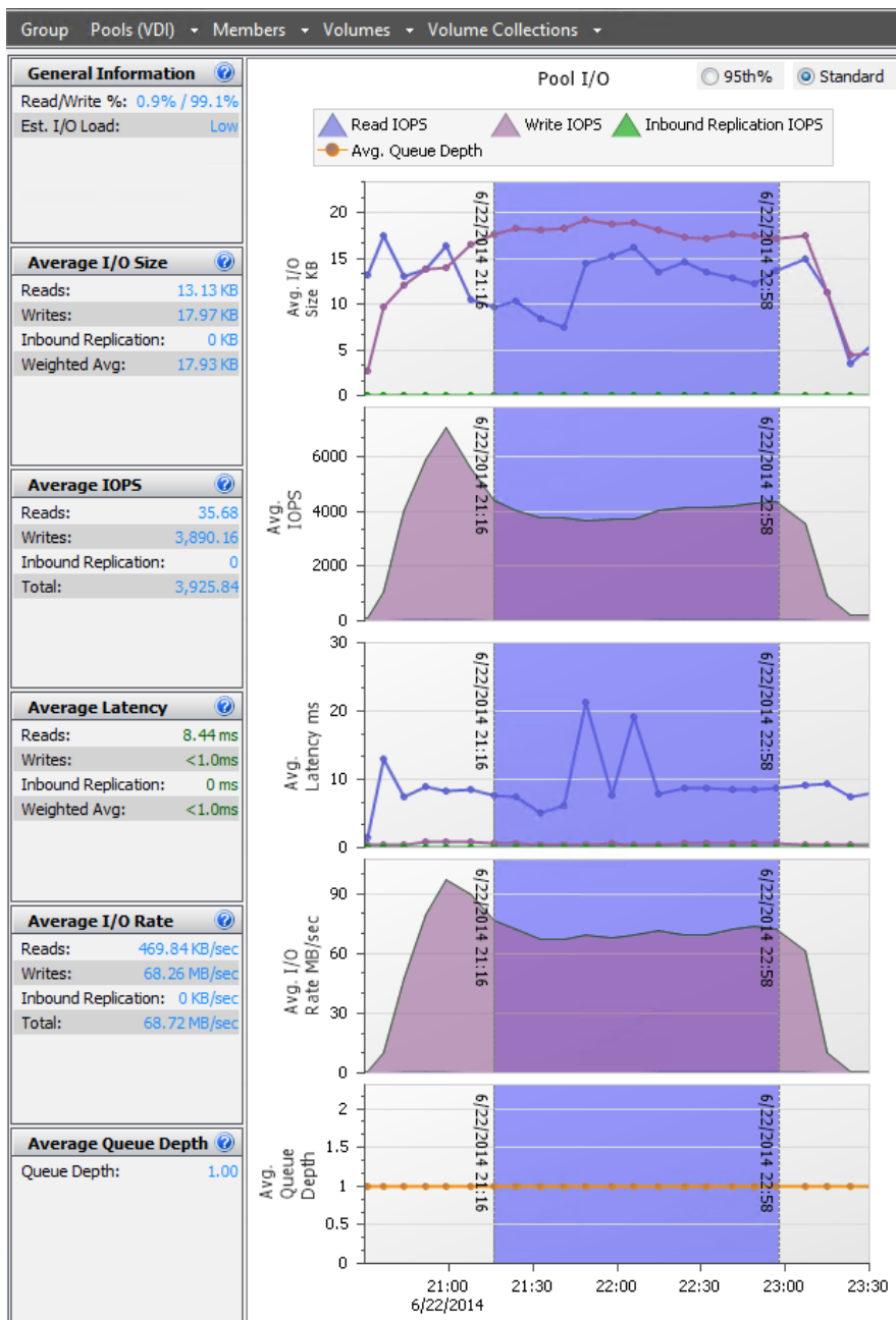
Figure 7 SAN HQ data showing steady state I/O for two PS-M4110XS arrays
