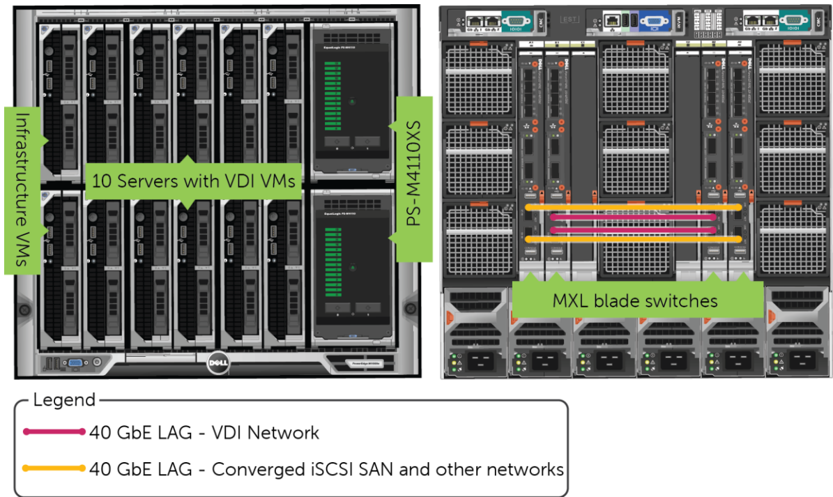
Figure 1 Compute, storage, and network layout in the PowerEdge M1000e blade chassis for the solution
