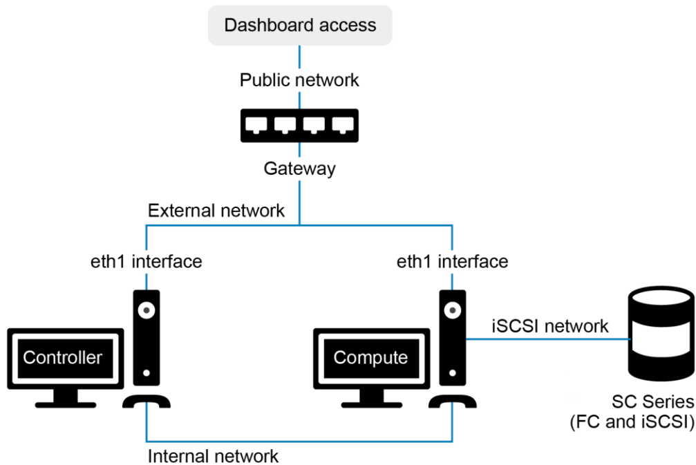
Figure 2 SC Series with OpenStack Cinder
