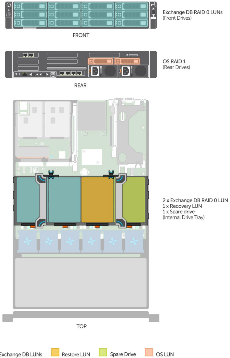
Figure 3. RAID LUN layout for the Exchange databases
